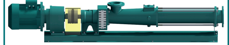
Housing bearing version Model: LK 065-1L
